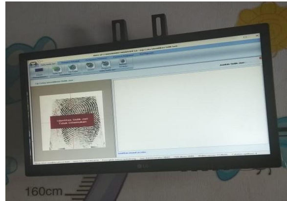
Gambar 5.2 Ujicoba Fingerprint
