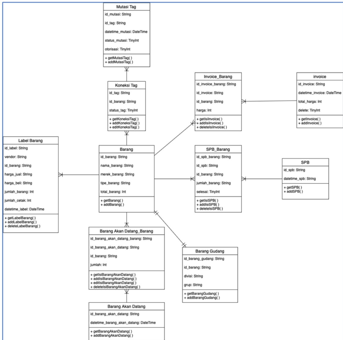
Gambar 2. Class diagram
